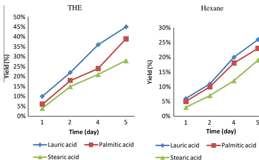
Figure 1 Effect of solvent and fatty chain length on acylation over Algerian bentonite.
