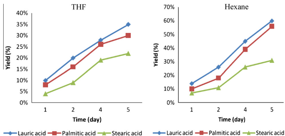
Figure 2 Effect of solvent and fatty chain length on the yield.
